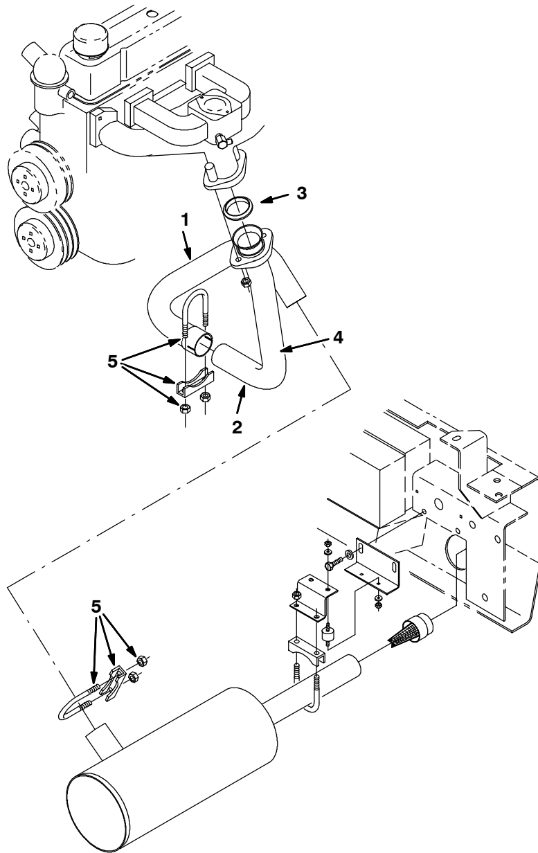
FIG. 1 - Exhaust Kit Installation
